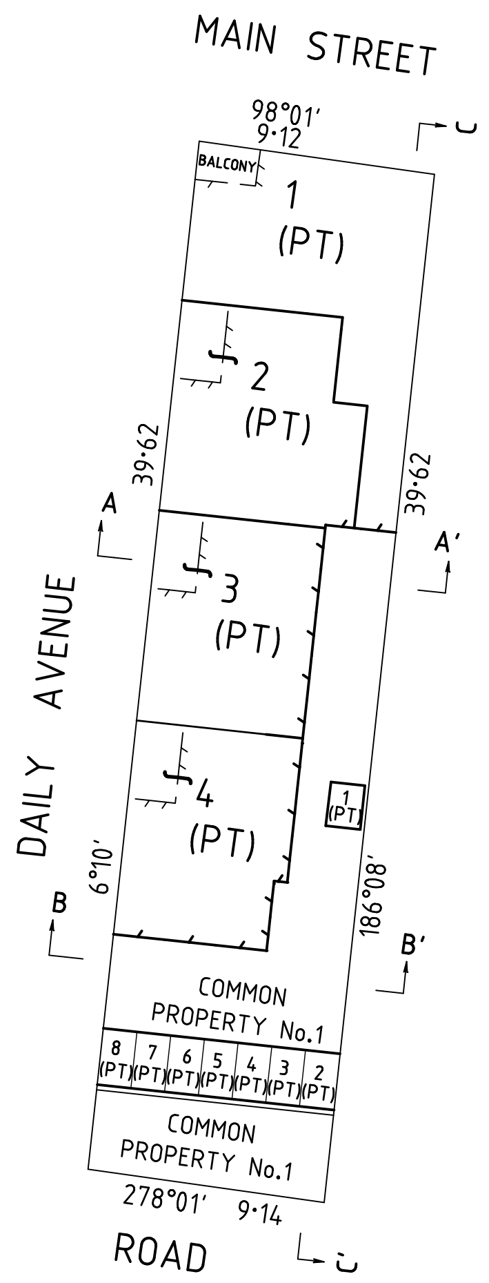
FIRST FLOOR DIAGRAM
